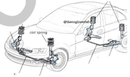
Suspension System
